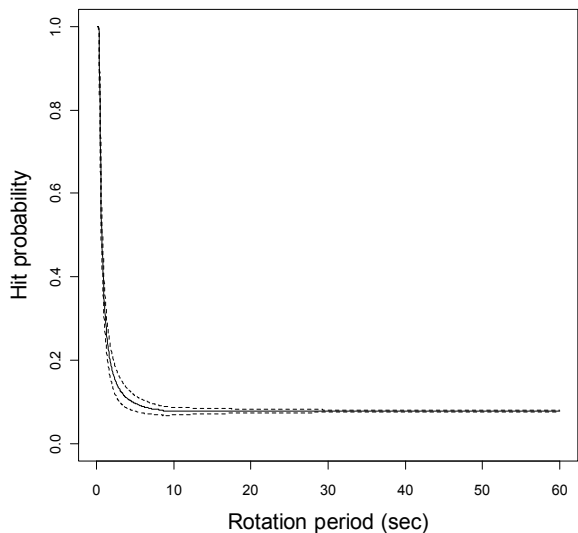
Figure 10. Hit probability for different RPM's of the wind turbine. Note that the minimum value never reaches zero (0.079); even when the turbine is standing still! The dotted lines indicate the probability for upwind (upper line) and downwind situations; the solid line indicates the mean of these two probabilities. This model was run using typical white-tailed eagle values: bird speed of 10.2 m/s ; bird length of 0.8 m; wingspan of 2.315 m. Turbine specifics were: pitch of 10°; max chord of 3.296m.
